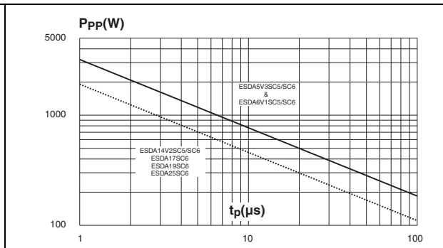
Figure 4. Peak pulse power versus exponential pulse duration ( T_j initial = 25\text{ }^{\circ}\text{C} )
