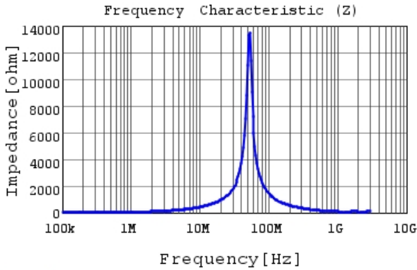
LQH32PN6R8NNC |Z|
