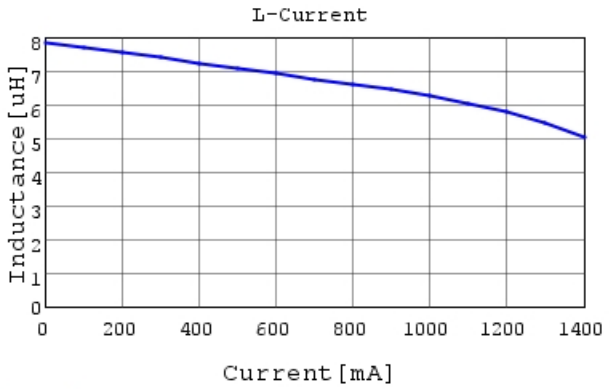
LQH32PN6R8NNC L-Current 20degC
