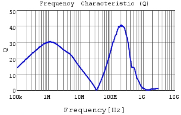
LQH32PN150MNC Q
