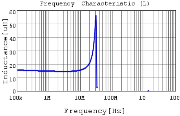
LQH32PN150MNC L
