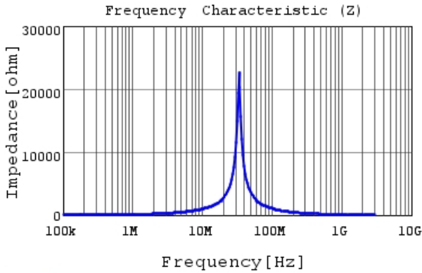
LQH32PN150MNC |Z|
