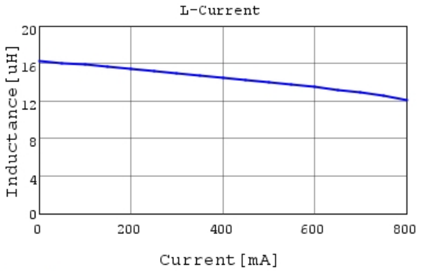
LQH32PN150MNC L-Current 20degC
