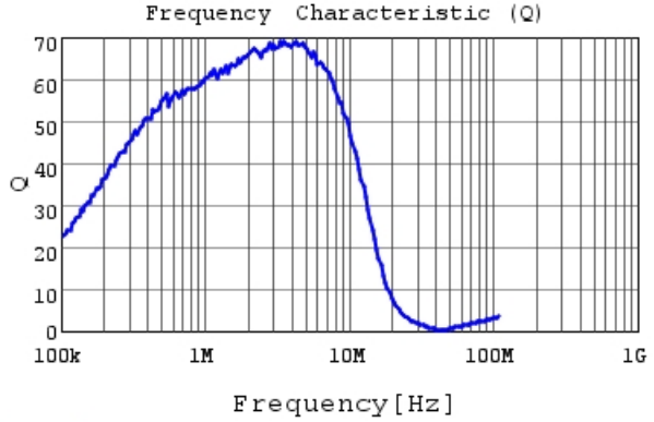
LQM2HPN3R3MG0 Q
