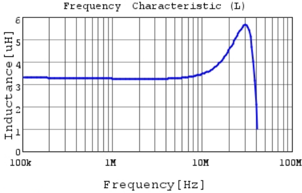
LQM2HPN3R3MG0 L
