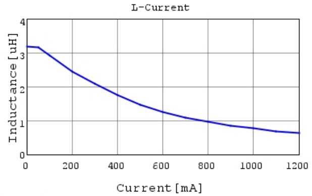
LQM2HPN3R3MG0 L-Current 20degC
