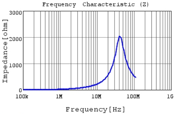
LQM2HPN3R3MG0 |Z|
