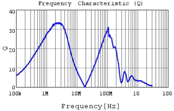
LQH2MCN820K02 Q
