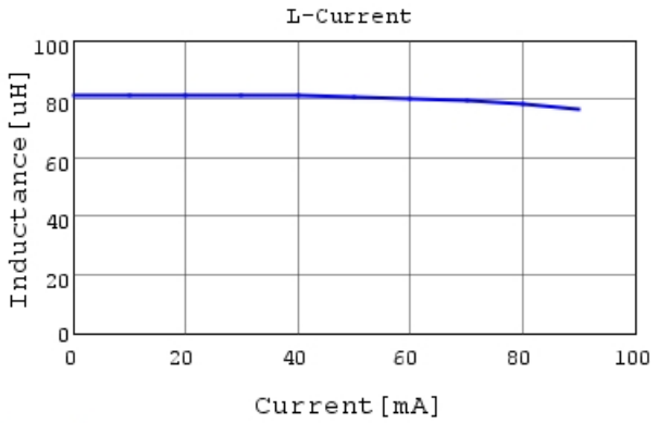
LQH2MCN820K02 L-Current 20degC
