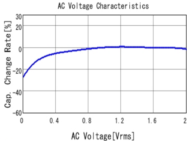
■ GRM033R61C224KE14 C-AC Voltage capchange, DCOV, 25.0d
