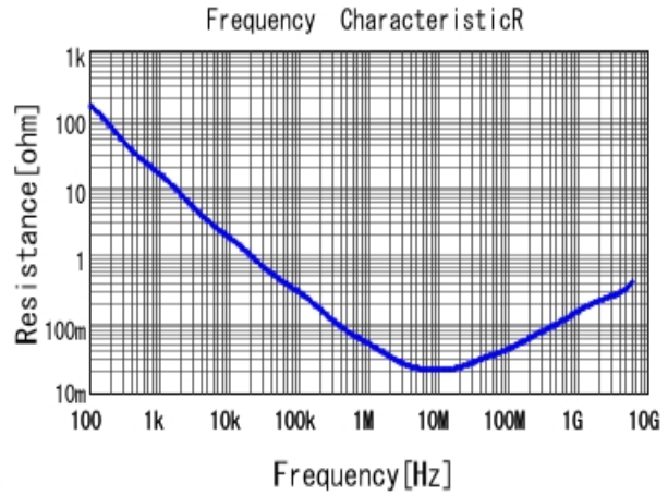
■ GRM033R61C224KE14 R DCOV, 25degC
