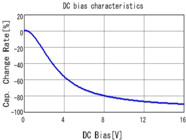
■ GRM033R61C224KE14 C-DC bias capchange, 25.0degC, AC1V
