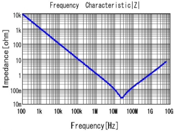
■ GRM033R61C224KE14 |Z| DCOV, 25degC
