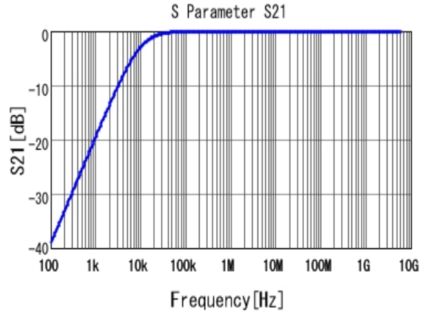
■ GRM033R61C224KE14 S21 DCOV, 25degC
