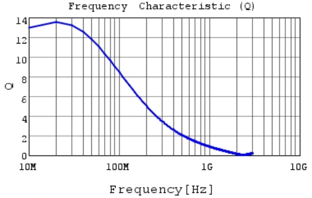
LQW18CNR12J00 Q
