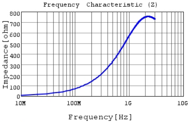
LQW18CNR12J00 |Z|
