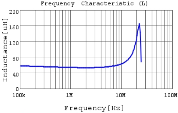
LQH2MCN560K02 L
