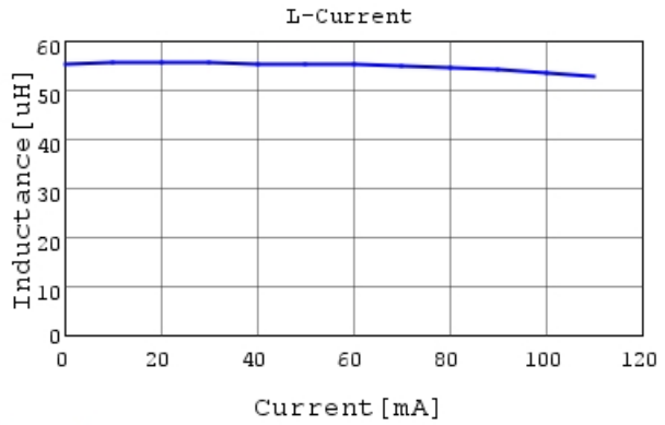
LQH2MCN560K02 L-Current 20degC
