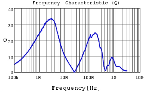
LQH2MCN560K02 Q
