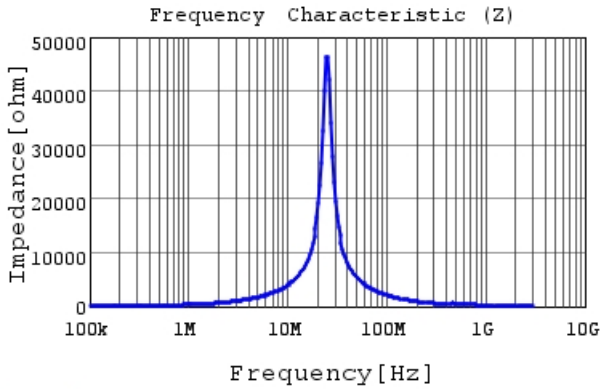
LQH2MCN560K02 |Z|
