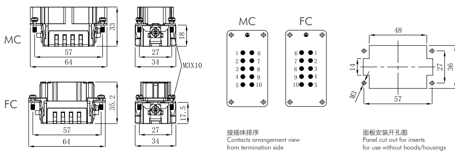
Dimensions mm
