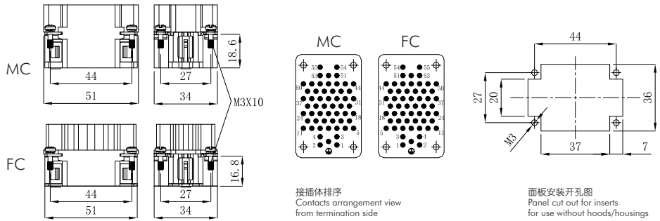
Dimensions mm
