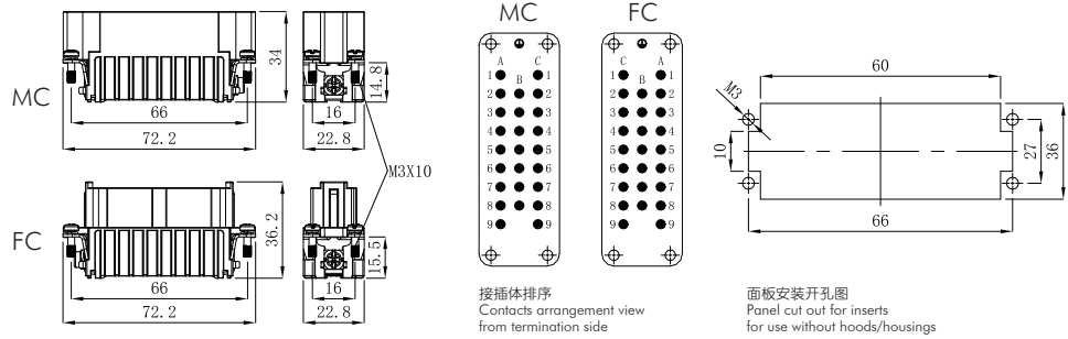
Dimensions mm
