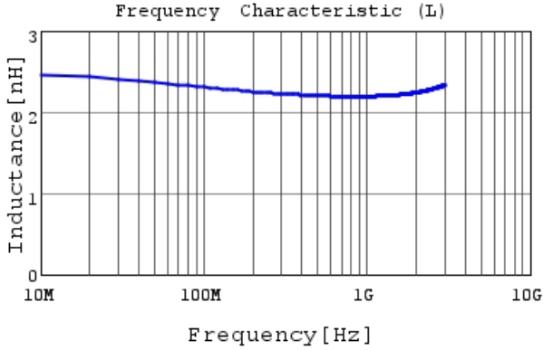
LQP03TN2N2B02 L
