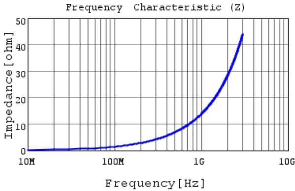
LQP03TN2N2B02 |Z|
