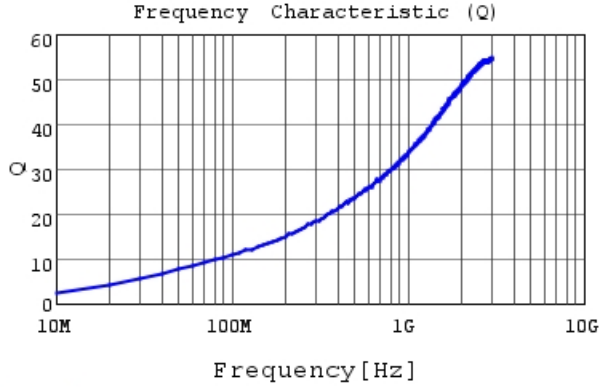
LQP03TN2N2B02 Q
