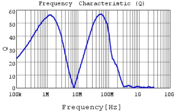
LQH43PN151M26 Q
