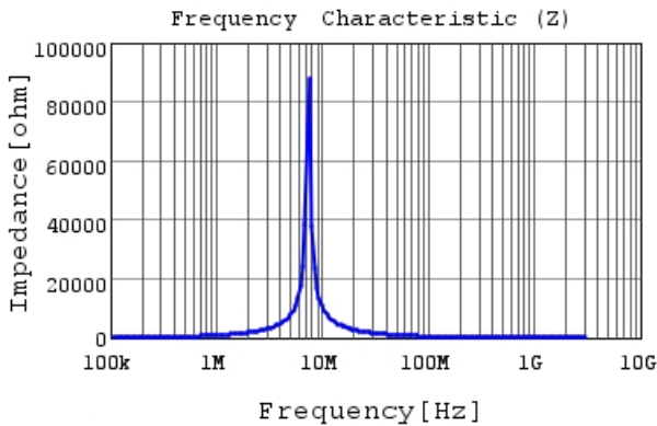
LQH43PN151M26 |Z|
