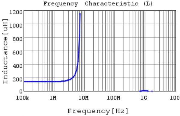
LQH43PN151M26 L
