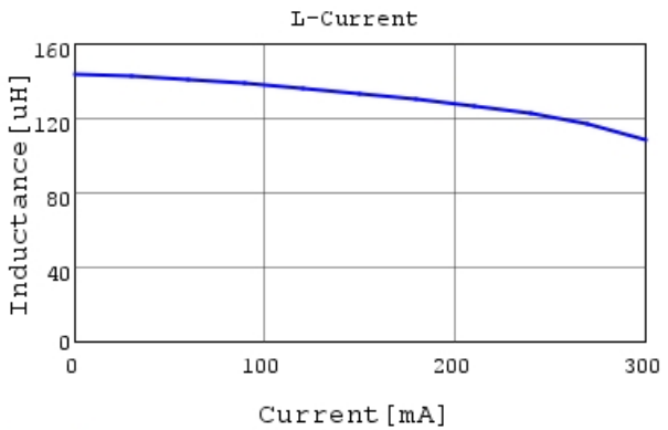
LQH43PN151M26 L-Current 20degC
