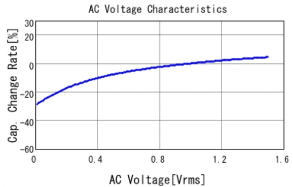
■ GCM21BM8EE106KE08 C-AC Voltage capchange, DC0V, 25.0d
