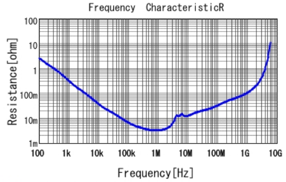
■ GCM21BM8EE106KE08 R DC0V, 25degC
