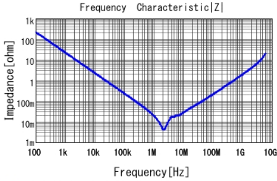
■ GCM21BM8EE106KE08 |Z| DC0V, 25degC
