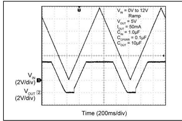
FIGURE 2-23: V_{IN} UVLO Threshold.
